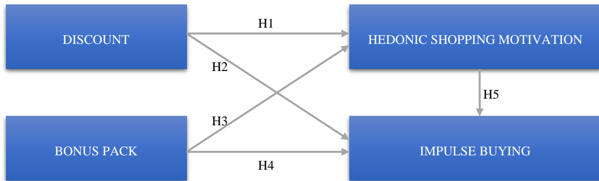
FIGURE 1. Framework
