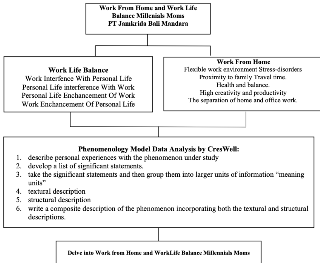
Figure 1. Research Framework
